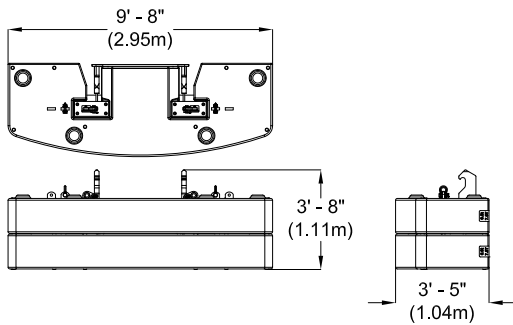
CONFIGURATION "B" WEIGHT: 30,000 lb (13607 kg)
