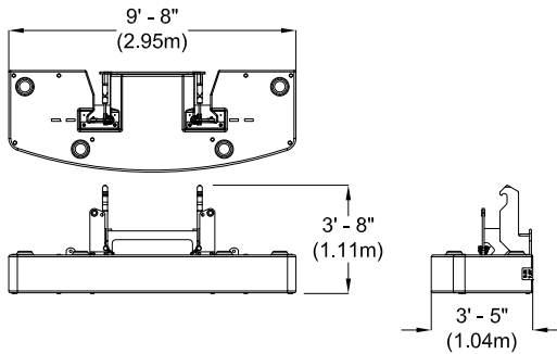
CONFIGURATION "A" WEIGHT: 15,000 lb (6804 kg)
